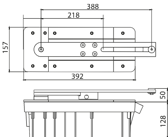
BOX/002 galvanized steel foundation box
